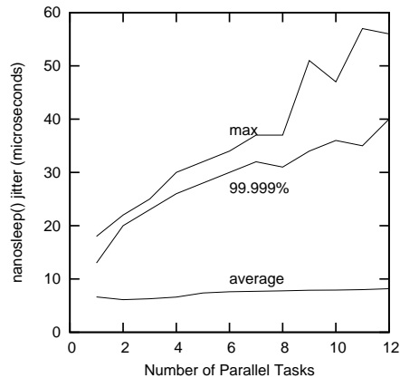
FIGURE 4: Nanosleep Jitter With Increased Load
