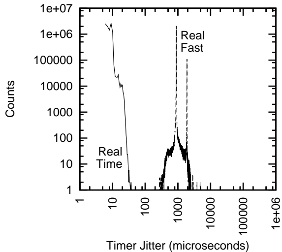
FIGURE 6: Real Time vs. Real Fast Timer Jitter
