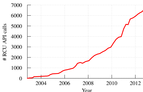
Figure 1: The number of uses of the RCU API in Linux kernel code from 2002 to 2013.
