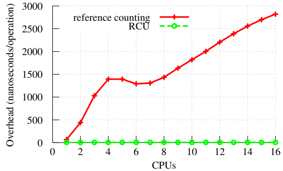
Figure 5: The overhead of entering using RCU as a reference count compared to the overhead of using a shared integer.
