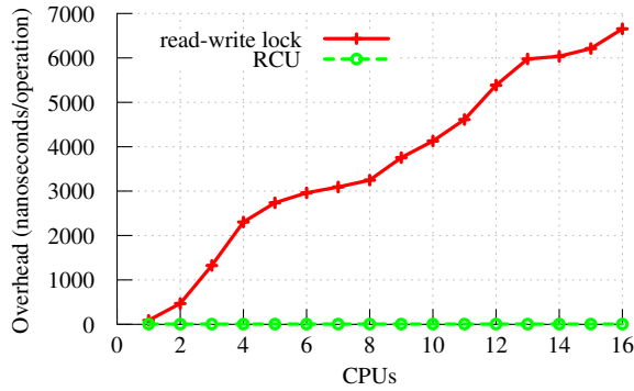
Figure 8: The overhead of entering and completing an RCU critical section, and acquiring and releasing a read-write lock.
